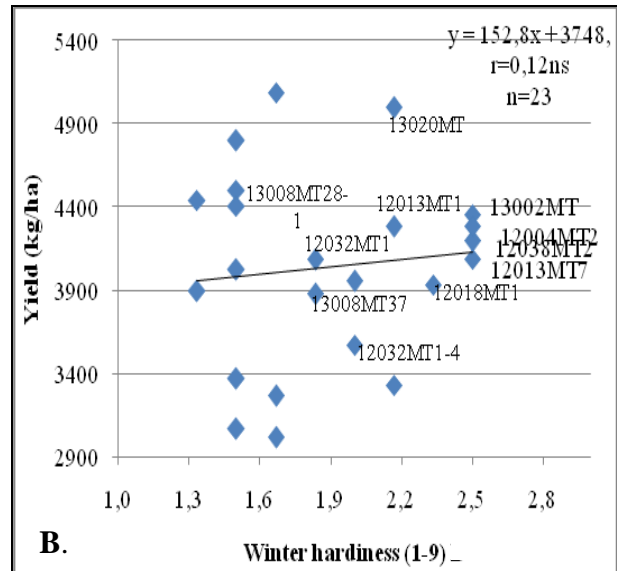
Figure 2. Relationships between winter hardiness and yield for 25 genotypes (A) and 23 genotypes of winter peas (B)
