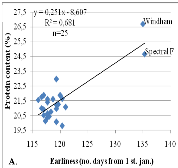
Figure 4. Relationships between the number of days from January 1 st till the end of flowering and protein content of 25 genotypes (A) and 23 genotypes winter peas (B)
