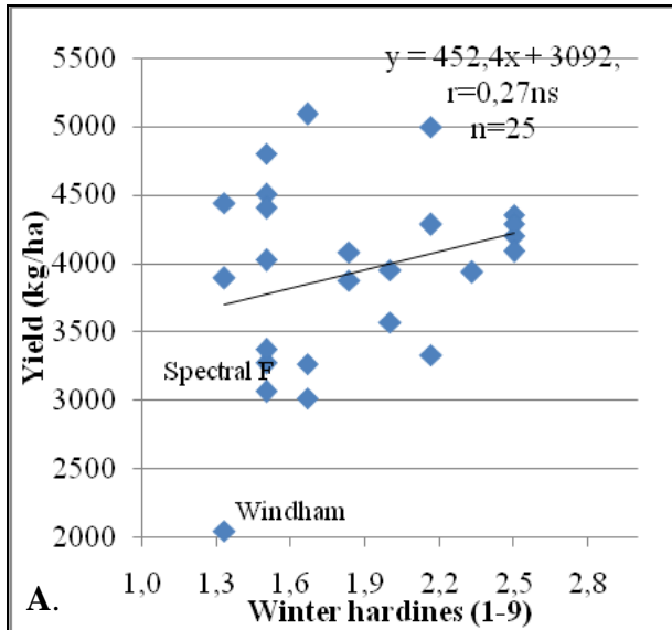
Figure 2. Relationships between winter hardiness and yield for 25 genotypes (A) and 23 genotypes of winter peas (B)
