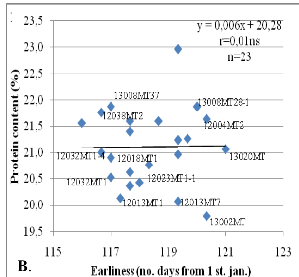
Figure 4. Relationships between the number of days from January 1 st till the end of flowering and protein content of 25 genotypes (A) and 23 genotypes winter peas (B)
