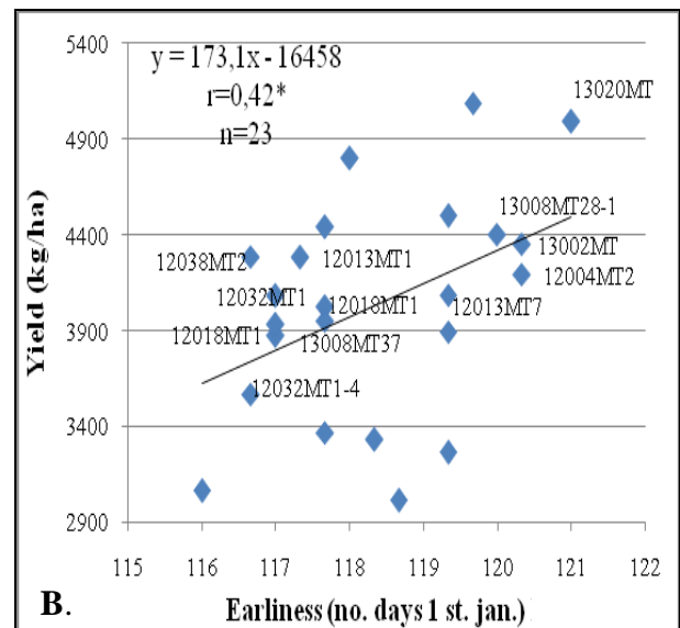
Figure 1. Relationships between earliness and yield of 25 genotypes (A) and 23 genotypes winter peas (B)
