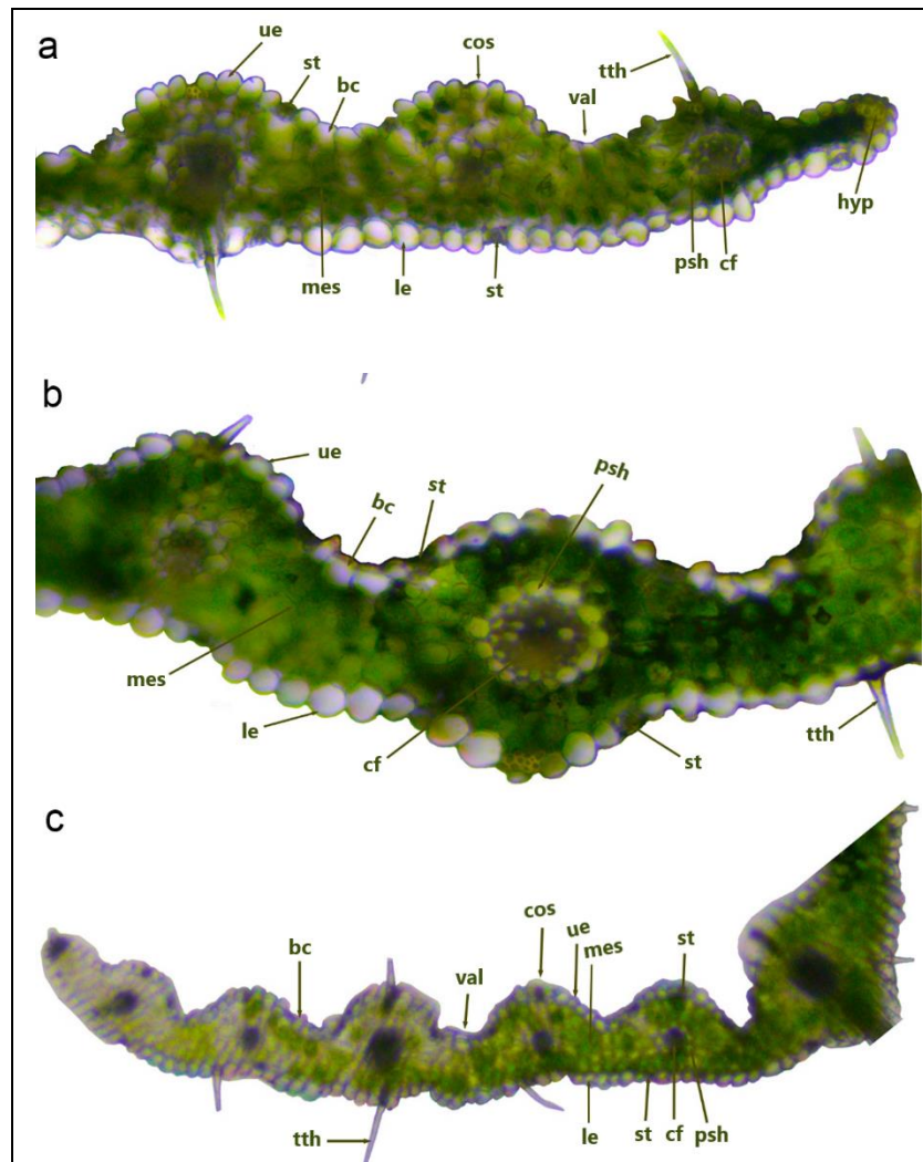
Figure 3. Leaf section
