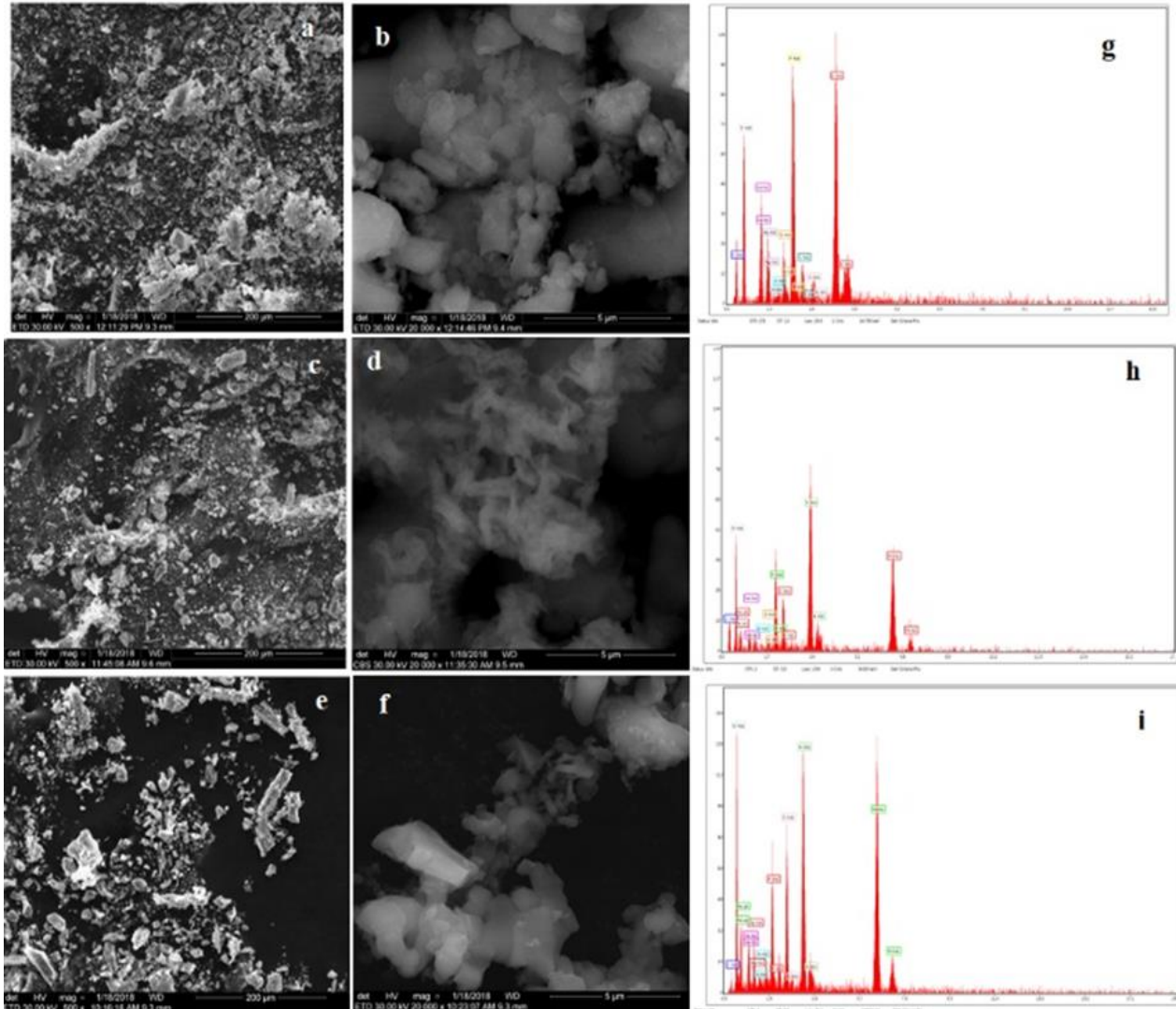
Figure 2. SEM images and EDX Spectrum
