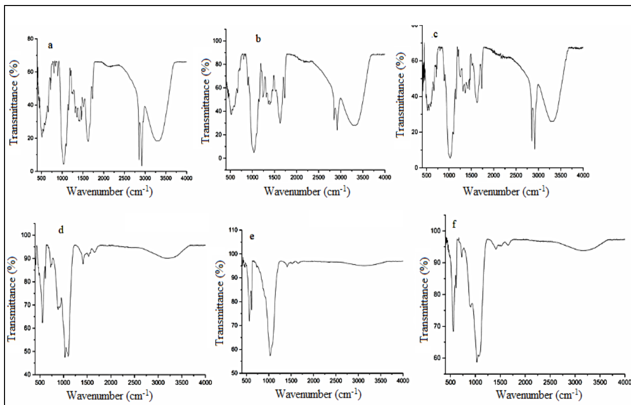
Figure 1. FTIR spectra of dried wheat leaves (a) control plants; (b) soil (root zone) fertilized plants with iron oxide solution during the growth process; (c) foliar fertilized plants with iron oxide solutions during the growth process; FTIR spectra of the calcined wheat plants samples at 650°C; (d) control plants; (e) soil (root) fertilized plants with iron oxide solution during the growth process; (f) foliar fertilized plants with iron oxide solutions during the growth process
